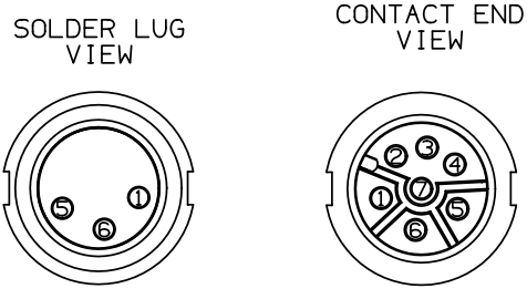
7 PIN MALE LOWRANCE CONNECTOR
