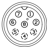
5/8 PIN FEMALE CONNECTOR #05-774-04
