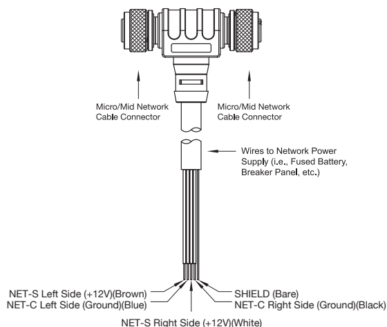
FIGURE 5. Micro/Mid Powertap
