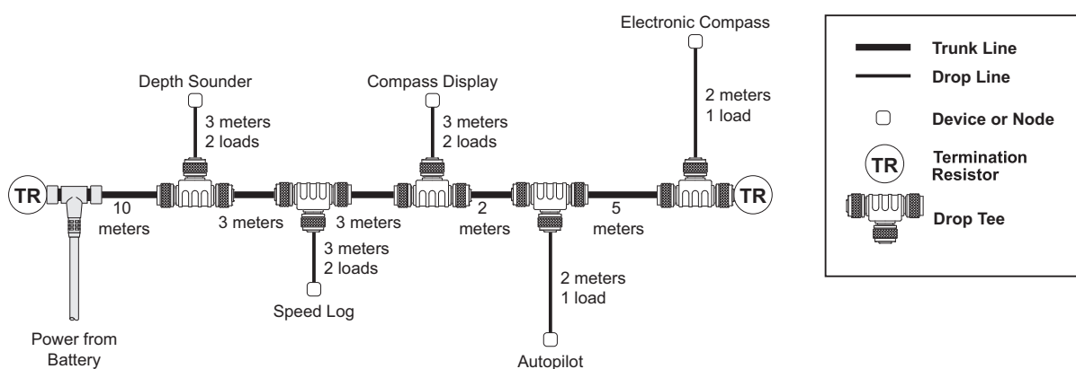
FIGURE 6. End-Powered Network
