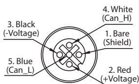
FEMALE END VIEW
