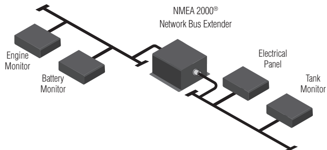
Network Extension End-to-End Example
