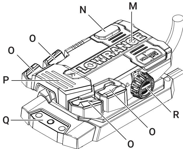
Foot pedal
