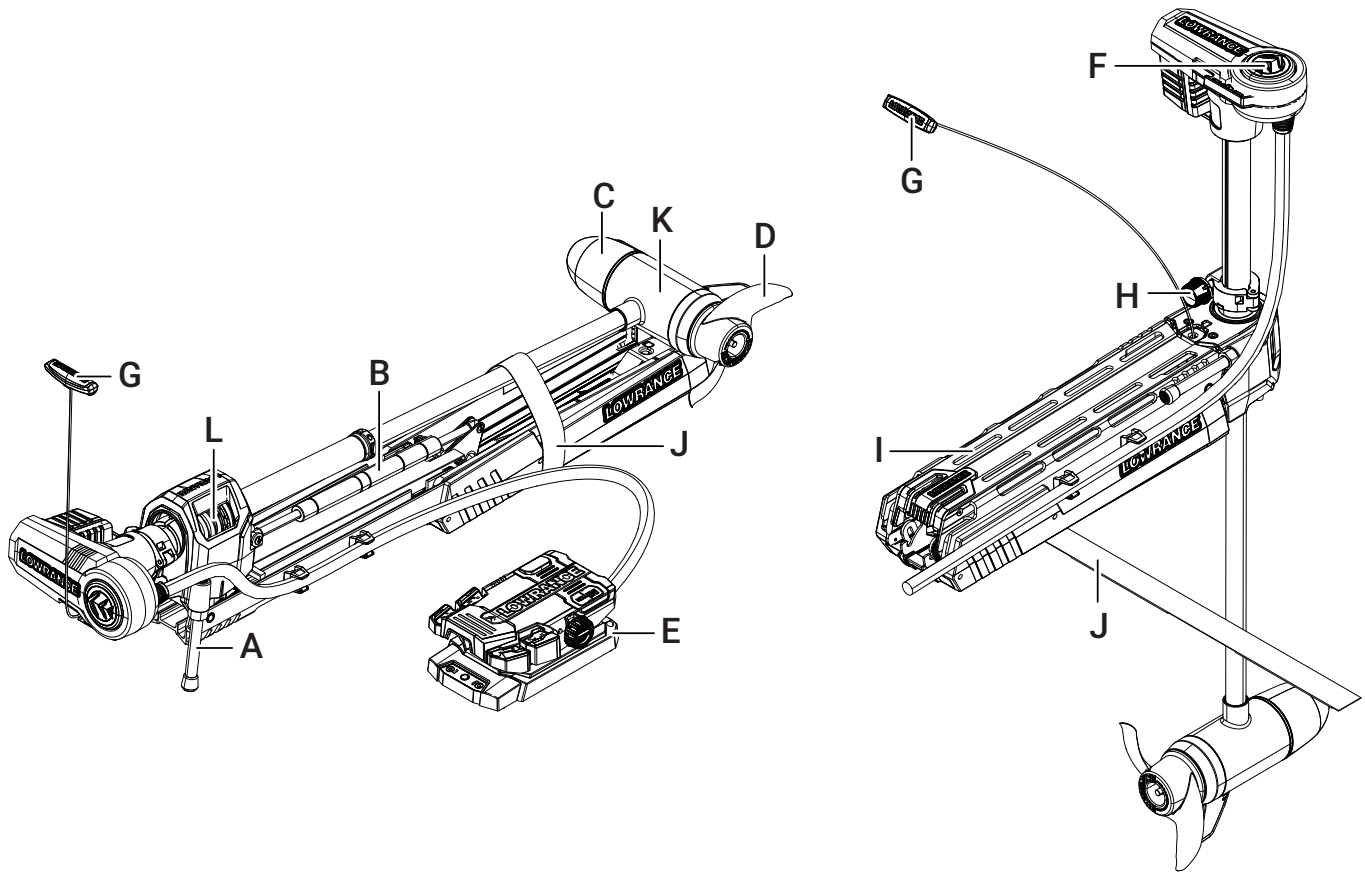
Stowed position
