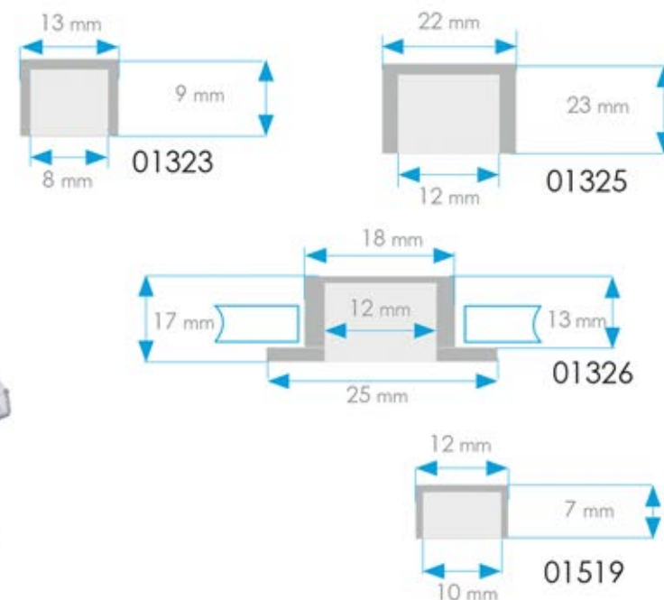
Encastré / Recessed
